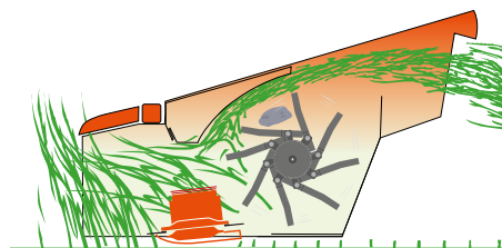
It requires a weight of 48.5lbs on the tine to pivot the SemiSwing tine backwards.
